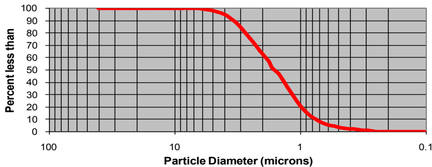
ImerSeal 75 - MicroTrac PSD Curve
